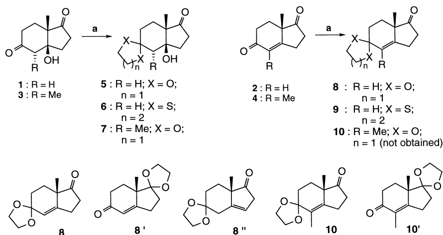
Scheme 2. Reagents and conditions: (a) \text{HO}(\text{CH}_2)_2\text{OH} , \text{BF}_3 \cdot \text{OEt}_2 or \text{TMSO}(\text{CH}_2)_2\text{OTMS} , \text{TMSOTf} , \text{CH}_2\text{Cl}_2 , -50^\circ\text{C} or \text{HS}(\text{CH}_2)_3\text{SH} , \text{BF}_3 \cdot \text{OEt}_2 , rt.
