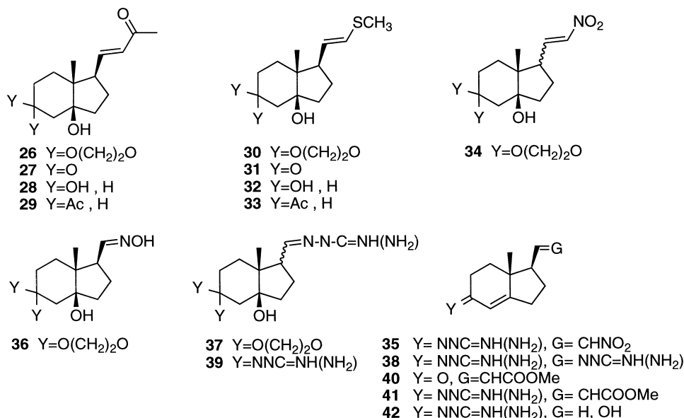
Figure 4. Synthesized molecules with hydroindene skeleton.
