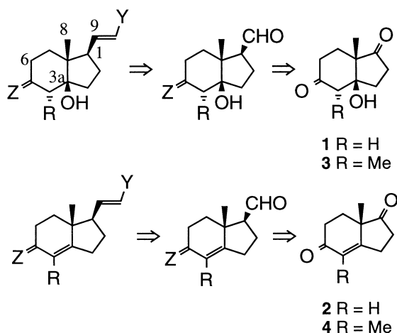
Scheme 1. Retrosynthetic analysis for planned hydroindenenes.
