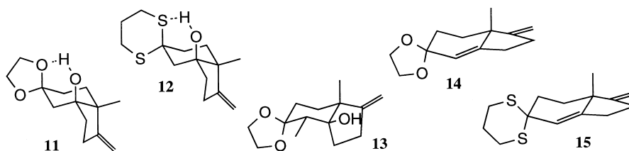
Figure 3. Preferred conformations of compounds 11–15 , from MM calculations and NMR data.
