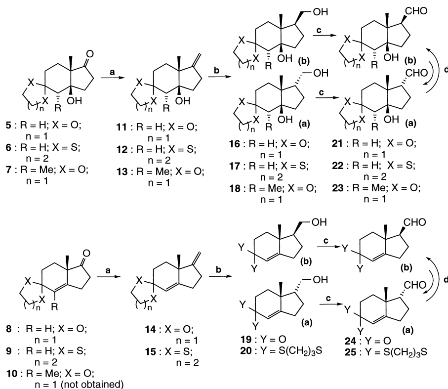
Scheme 3. Reagents and conditions: (a) (\text{C}_6\text{H}_5)_3\text{P} + \text{CH}_3\text{I}^- , \text{NaOtAm} , \text{C}_6\text{H}_6 , reflux; (b) 1. \text{BH}_3/\text{THF} or 9-BBN, rt; 2. \text{H}_2\text{O}_2 , \text{NaOH} , \text{EtOH} , 50^\circ\text{C} ; (c) \text{CCP} , \text{CH}_2\text{Cl}_2 , rt; (d) \text{KOH}/\text{EtOH} 5%, rt.
